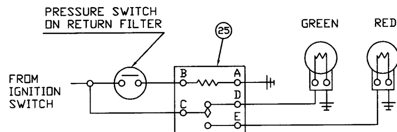
WIRING DIAGRAM
