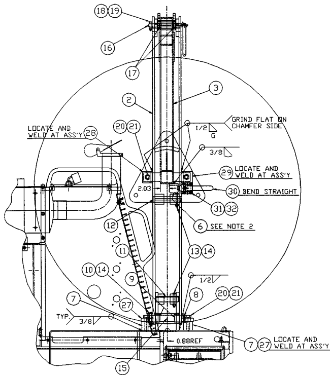
1 ASSEMBLY
